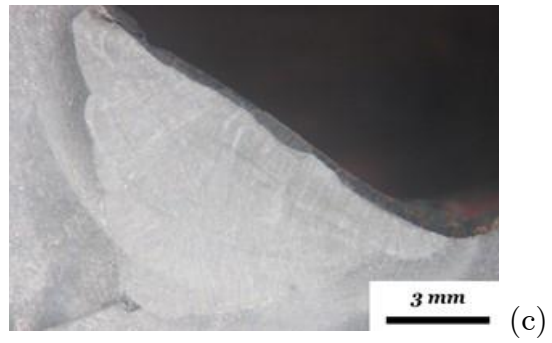
Figure 50. (a) Macrostructure of a typical L-joint welded specimen; (b), (c) detail the macrostructure, showing the WM, HAZ and BM.
